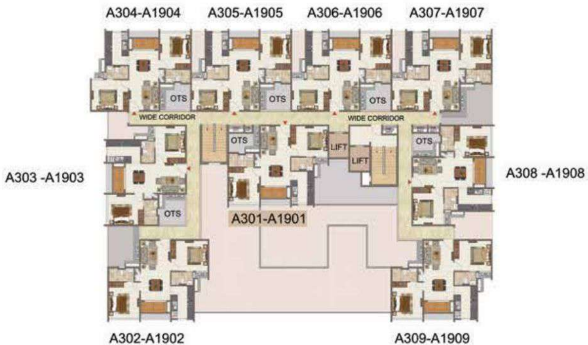
TYPICAL FLOOR PLAN (3RD TO 19TH FLOOR)
